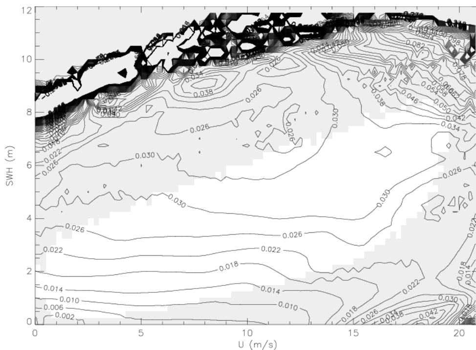
Figure 17: Difference of SSB computed with EIGEN-GRACE and DGME-04 orbits
