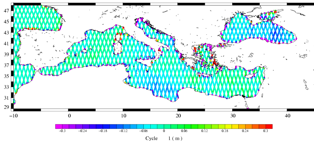
Figure 33: Height difference between the new and old mean profiles over the Mediterranean Sea
