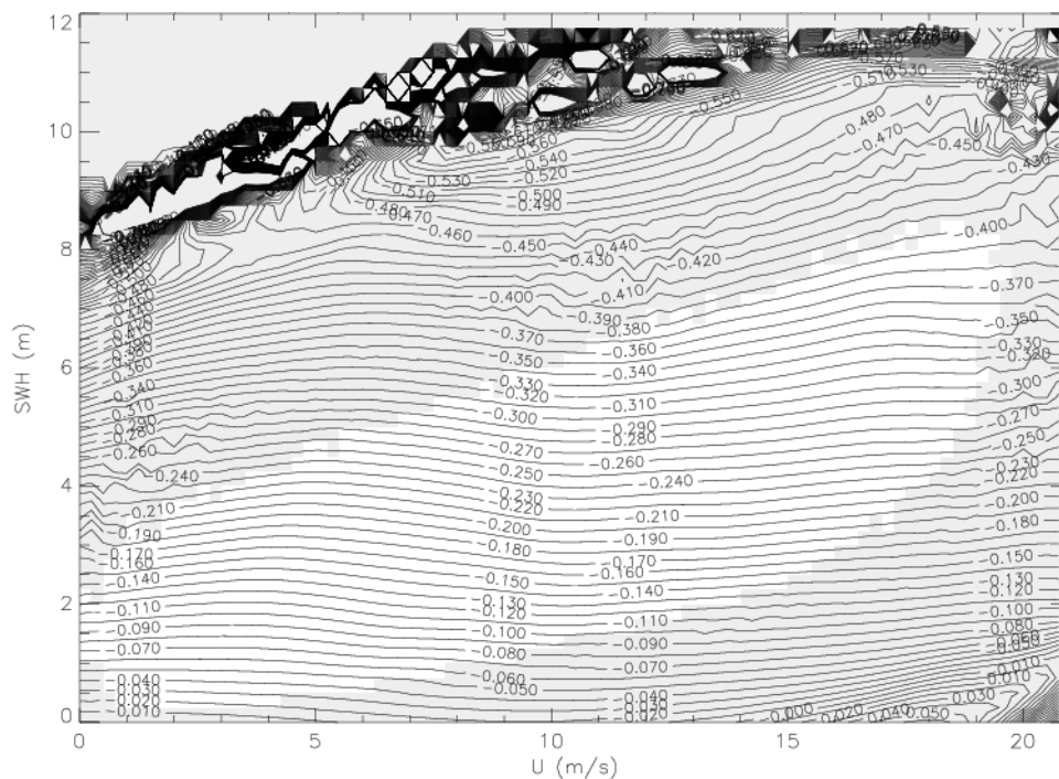
Figure 11: SSH estimation using EIGEN-GRACE01S orbit and new corrections in SSH
