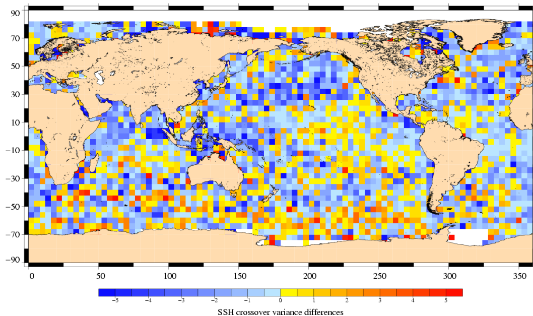
Figure 27: difference of variance ( cm^2 ) at crossovers
