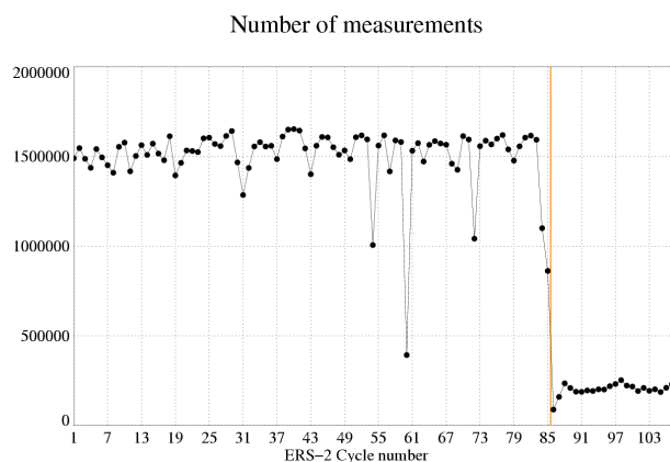
Figure 1: Number of edited measurements for cycles 1 to 98
