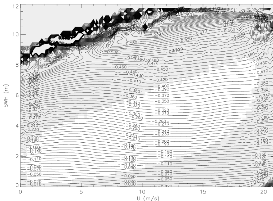
Figure 9: SSB estimation with spline interpolation and (3m/s,1.5m) window parameter
