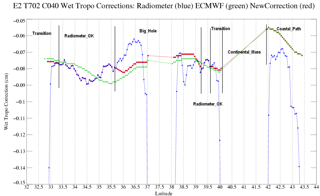
Figure 31: Radiometer, model and composite wet troposphere correction profiles for pass 702, cycle 040
