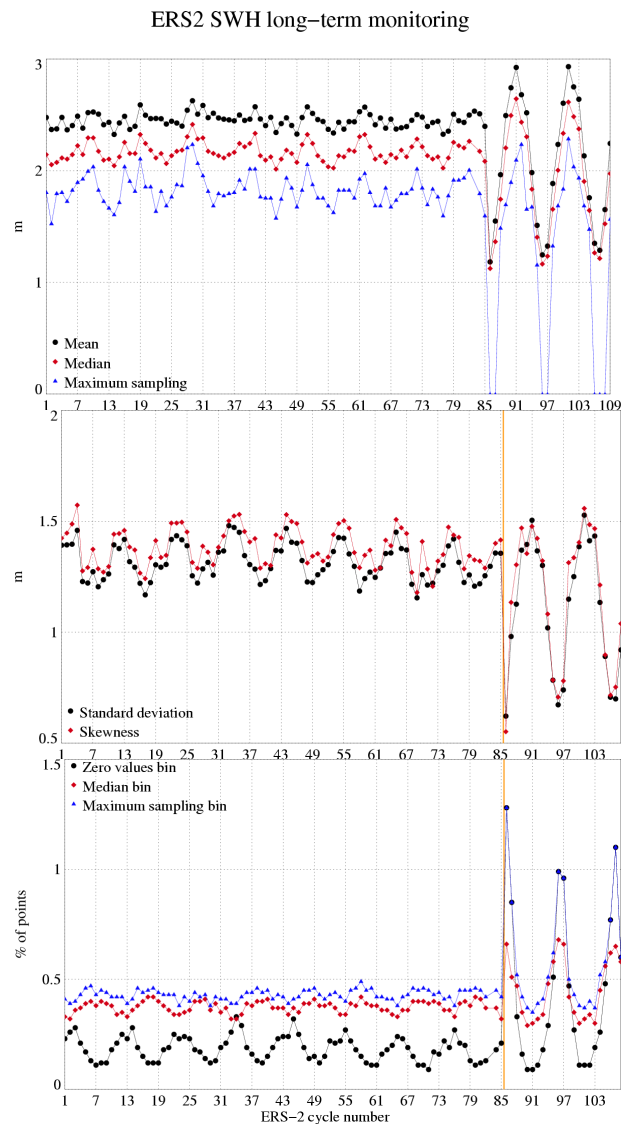
Figure 4: Statistical results on the ERS-2 OPR significant wave height
