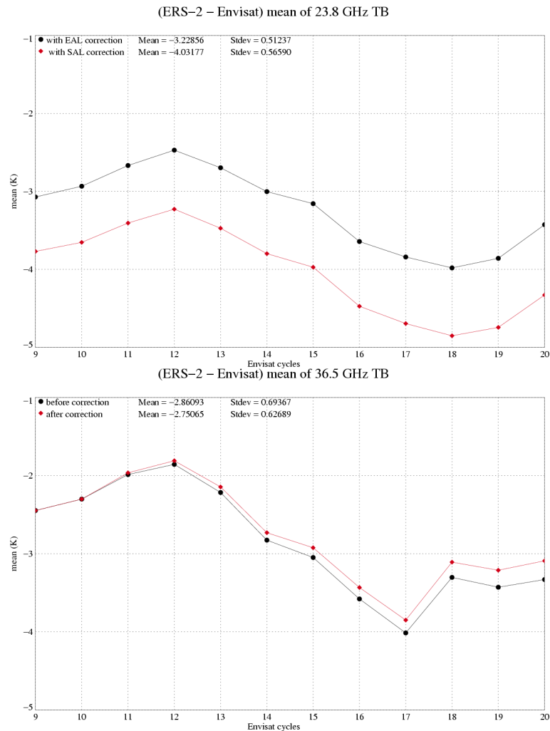
Figure 7: Mean of (ERS-2 - Envisat) TB 23.8 GHz(top) and TB36.5 GHz(bottom)
