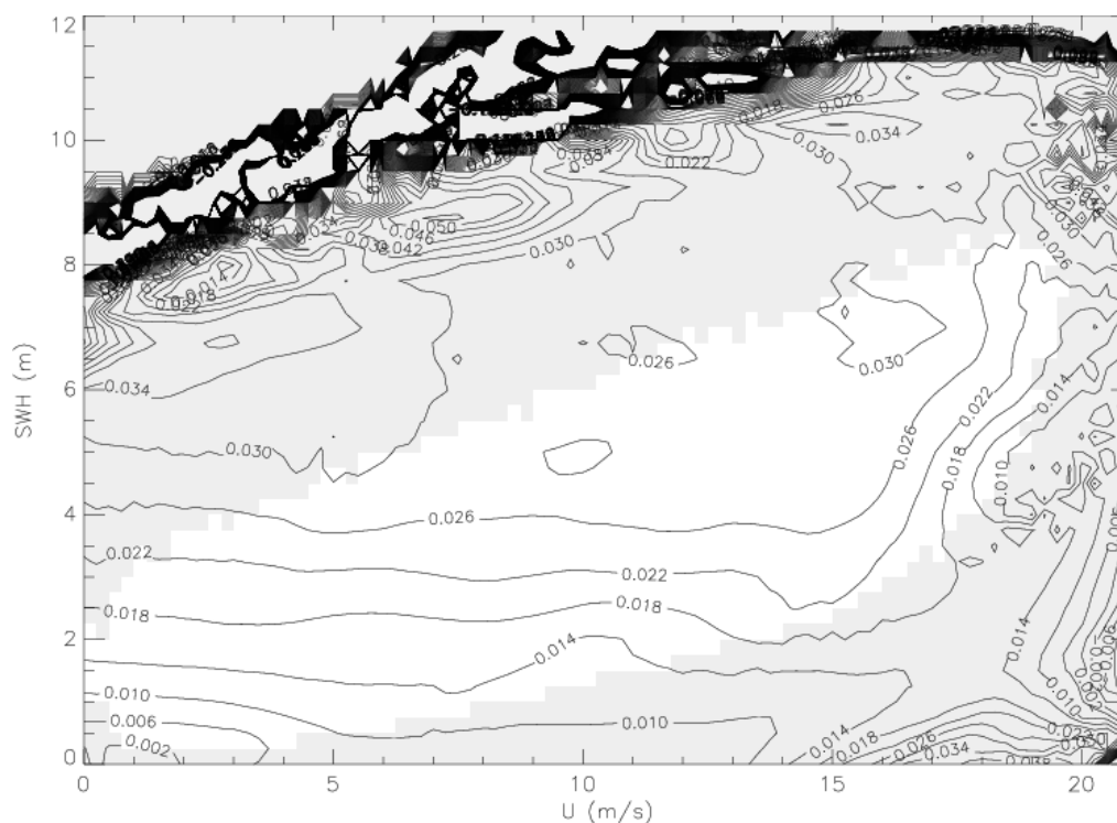
Figure 10: Difference of SSB estimate with and without spline filtering
