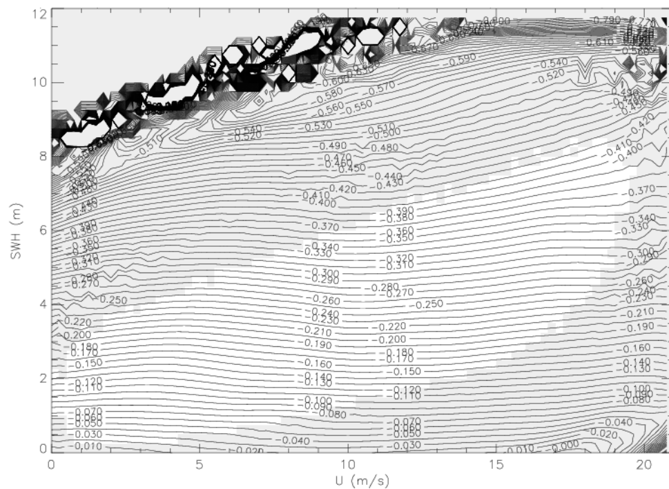
Figure 19: SSB estimation using EIGEN-GRACE orbit corrected for orbit error
