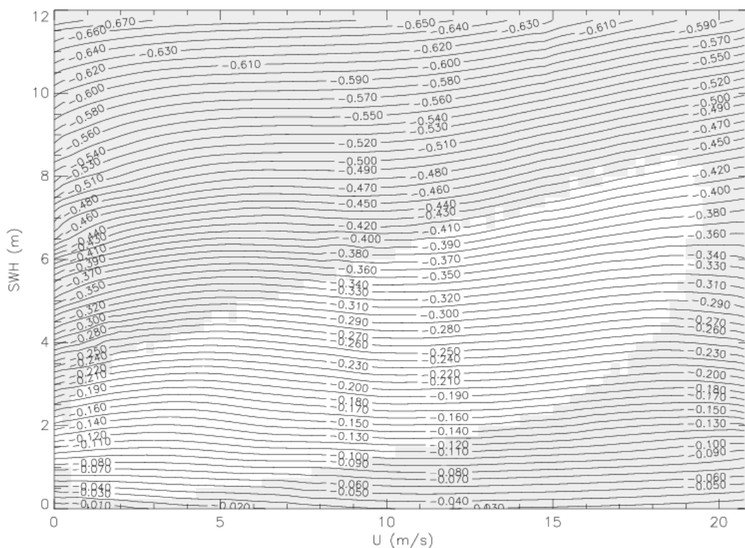
Figure 21: SSB estimation with the new smoothing factor
