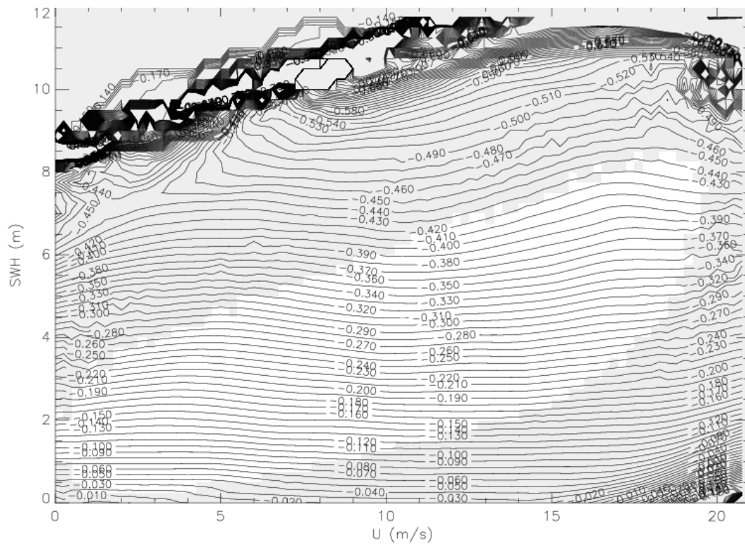
Figure 24: SSB estimate obtained with collinear method
