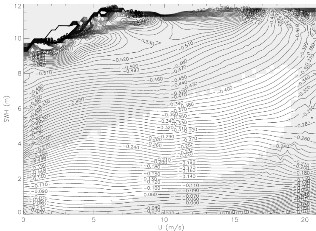
Figure 22: SSB estimate obtained with direct method
