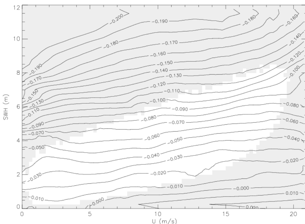
Figure 28: Difference of (Envisat - ERS-2) SSB estimates
