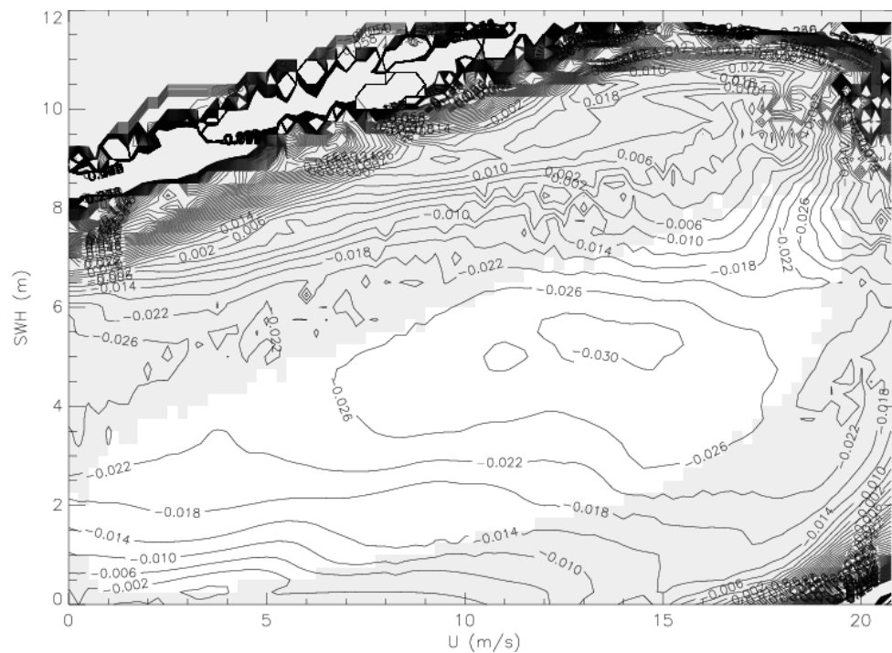
Figure 25: difference SSB collinear and crossover methods
