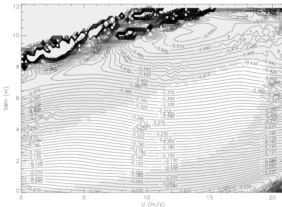
Figure 13: SSB estimation using EIGEN-GRACE orbit and old corrections in SSH
