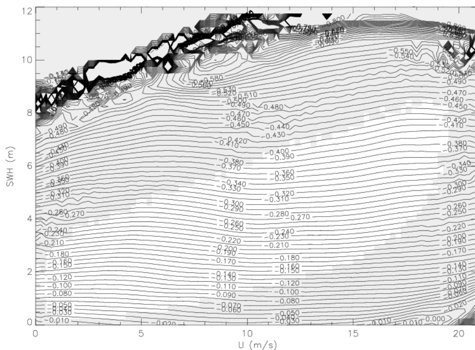
Figure 16: SSB estimation using DGME-04 orbit and new corrections in SSH
