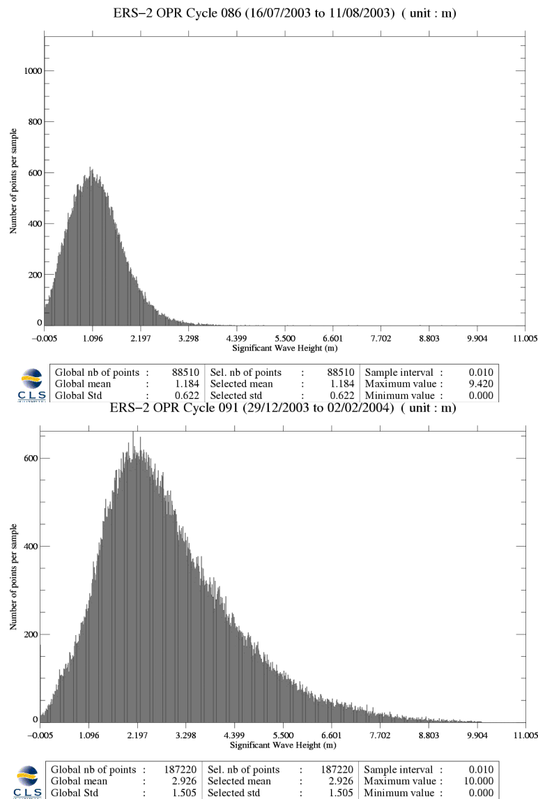
Figure 5: Histograms of the ERS-2 OPR significant wave height for cycles 86 and 91
