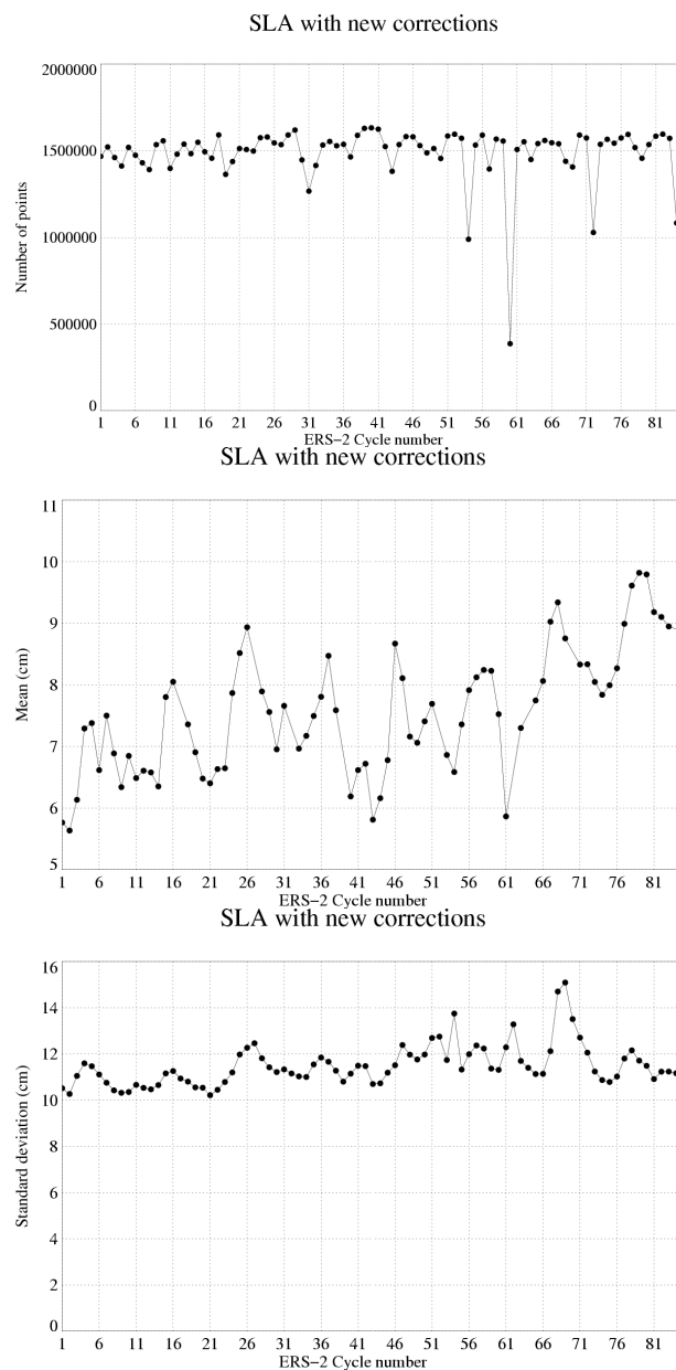
Figure 8: Cyclic number of points (top) mean (middle) and standard deviation (bottom) of SLA with new corrections applied
