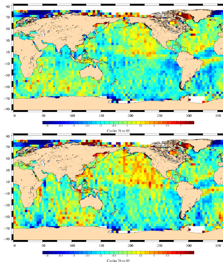
Figure 15: Mean of SSH crossovers with EIGEN-GRACE (top) and DGME-04 (bottom) orbits with new SSH
