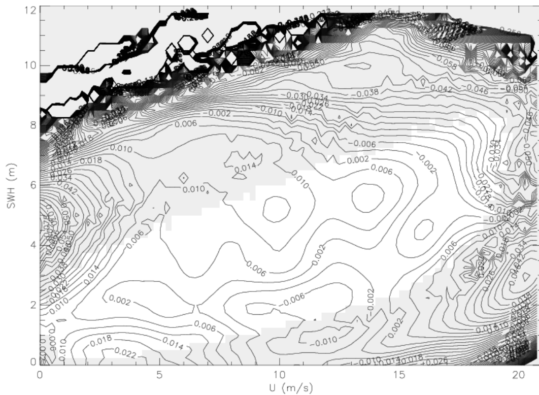
Figure 23: Difference SWH from direct and crossover methods
