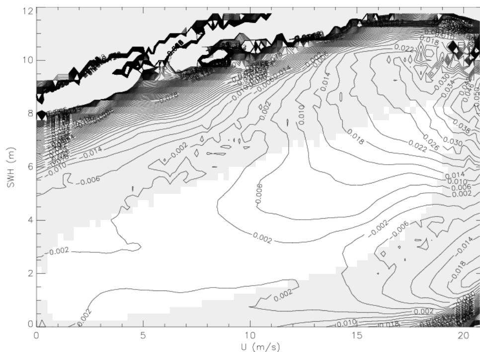
Figure 14: Difference of SSB computed with EIGEN-GRACE orbit and new and old corrections in SSH
