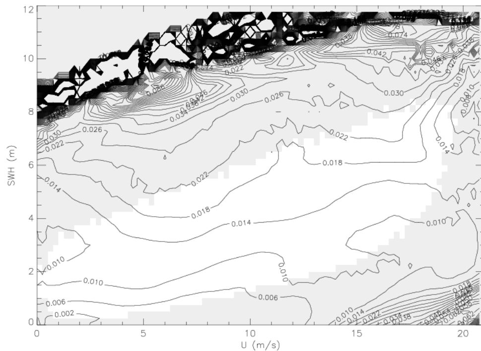
Figure 20: Difference of SSB using EIGEN-GRACE orbit with and without orbit error
