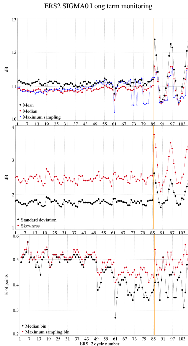
Figure 3: Statistical results on the ERS-2 OPR backscatter coefficient
