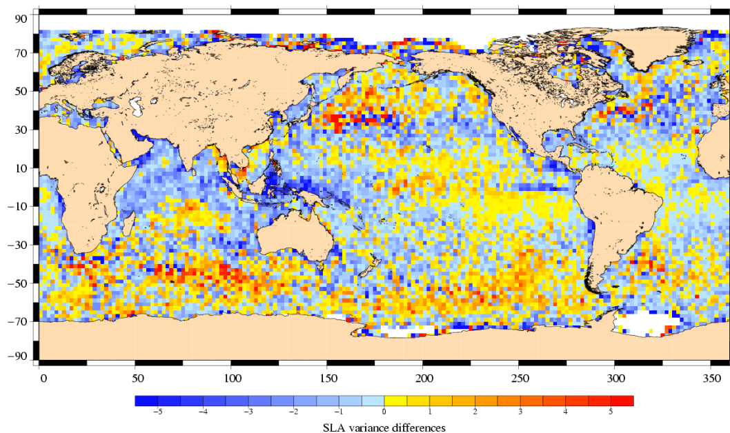
Figure 26: difference of variance ( cm^2 ) along-track
