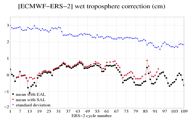
Figure 6: Mean and standard deviation of (ECMWF - ERS-2) wet troposphere correction
