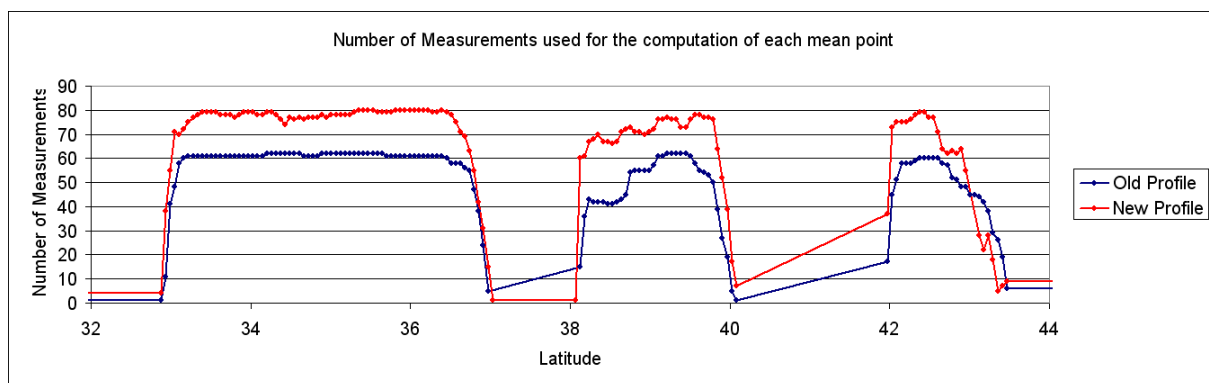
Figure 34: Number of measurements used in the computation of each point of the old and new mean profiles for pass 702 over the Mediterranean Sea
