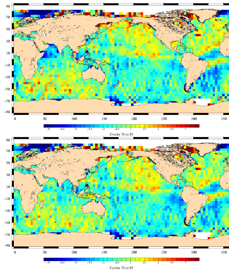
Figure 12: Mean of SSH crossovers with old (top) and new (bottom) corrections in SSH
