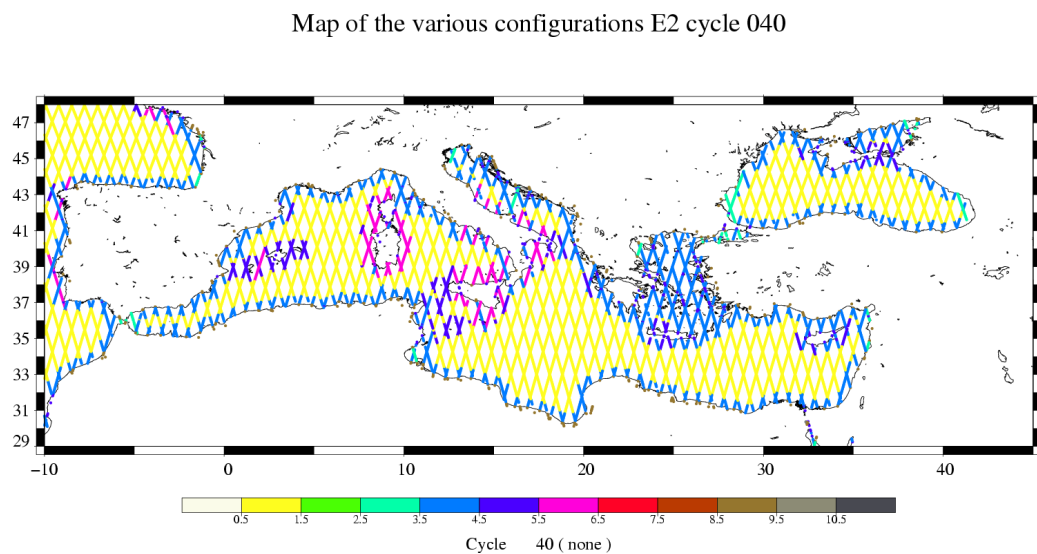
Figure 30: Configurations in Mediterranean Sea: 1=Radiometer_OK, 3=Coastal_Path, 4=Transition, 5=Small_Hole, 6=Big_Hole, 9=Continental_Mass, 10=Track_End
