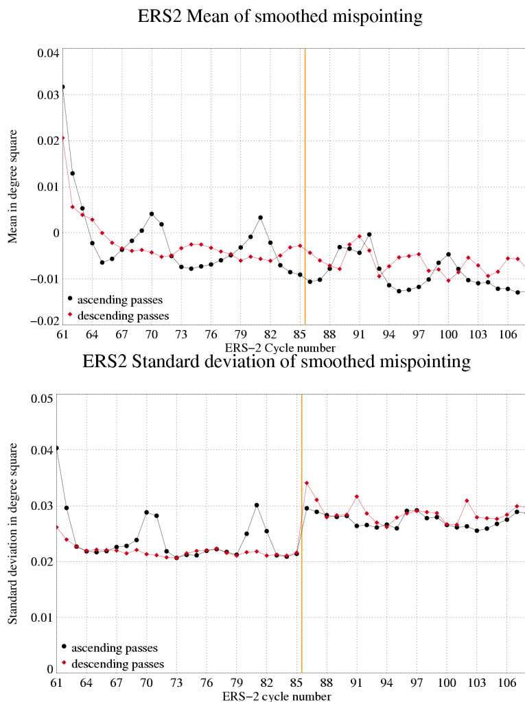
Figure 2: Cycle mean (top) and standard deviation (bottom) of mispointing for ascending and descending passes.
