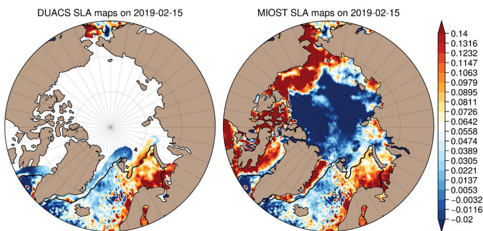
Figure 1: Gridded Sea Level Heights computed with (left) Duacs global product and (right) MIOST combining altimetry and drifters
